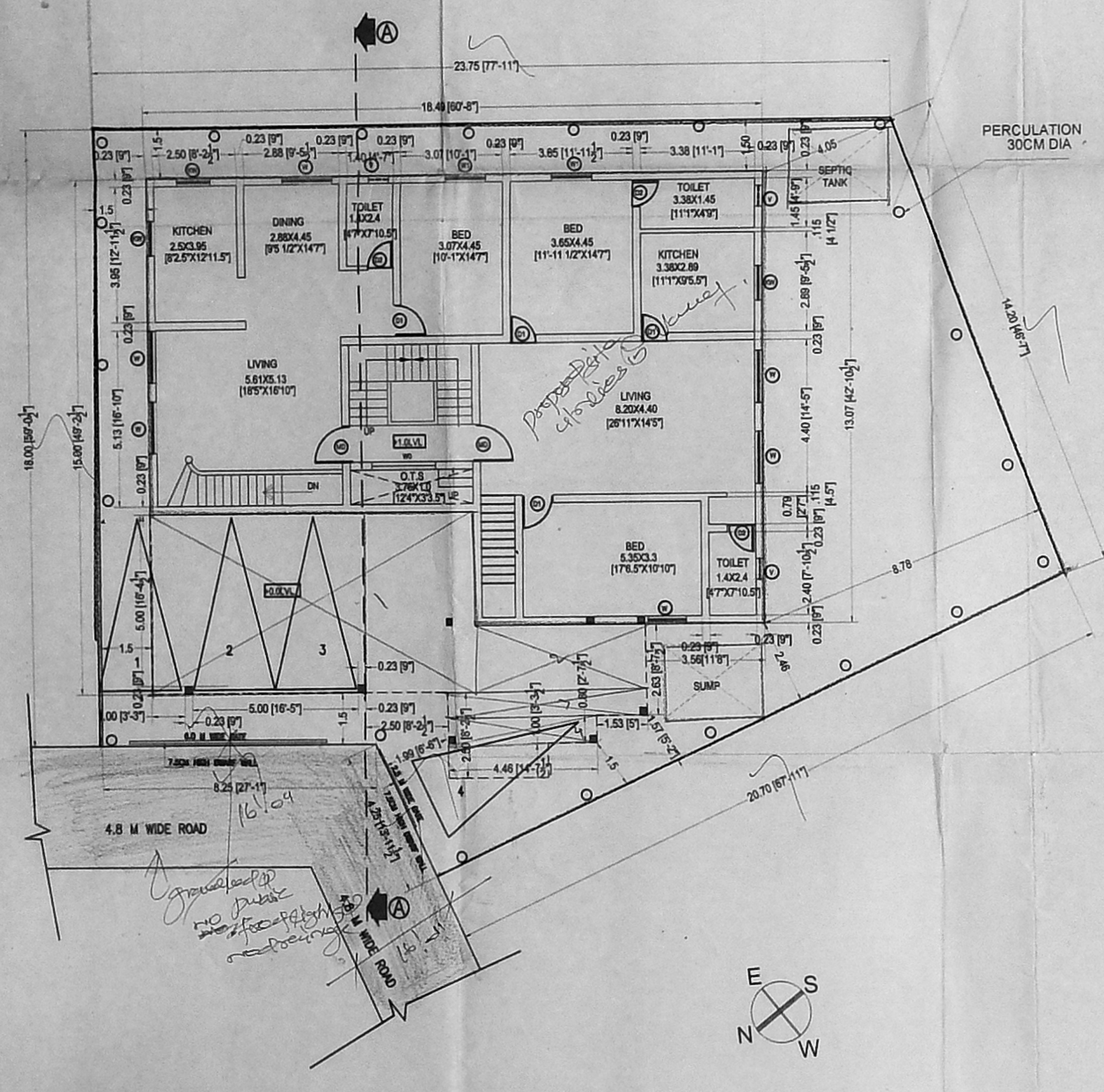
SITE CUM STILT AND GROUND FLOOR PLAN
